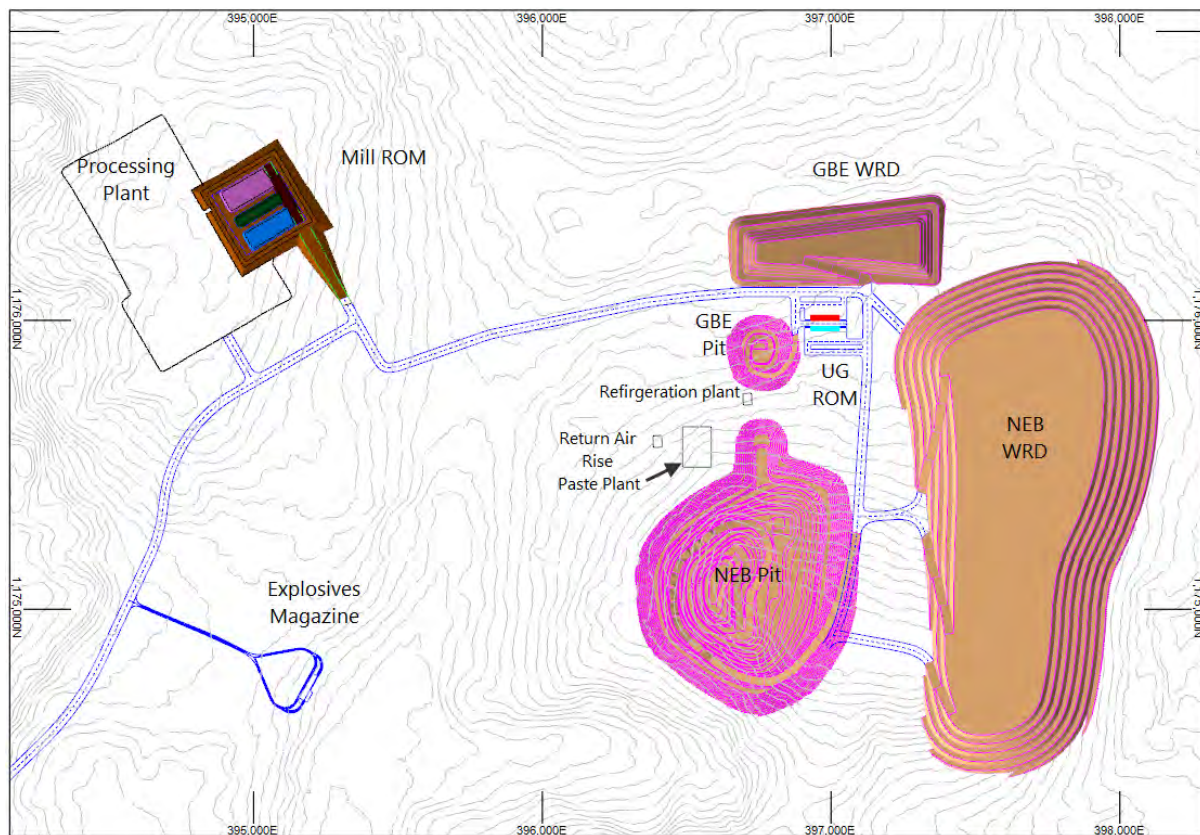
Figure 16.78: Surface Power Required Areas
