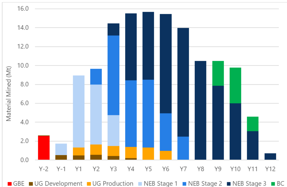
Figure 16.42: Project LOM Schedule – Total Material Mined
