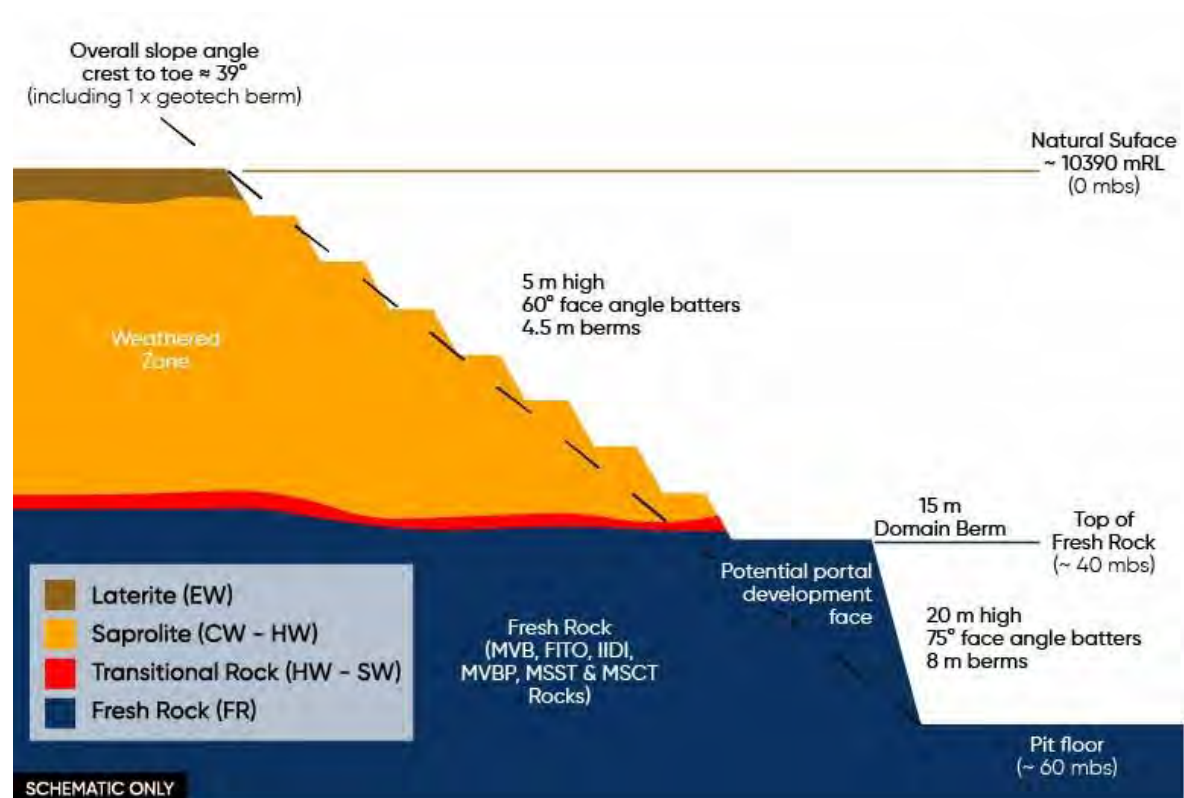
Figure 15.7: GBE Pit Wall Design Parameters
