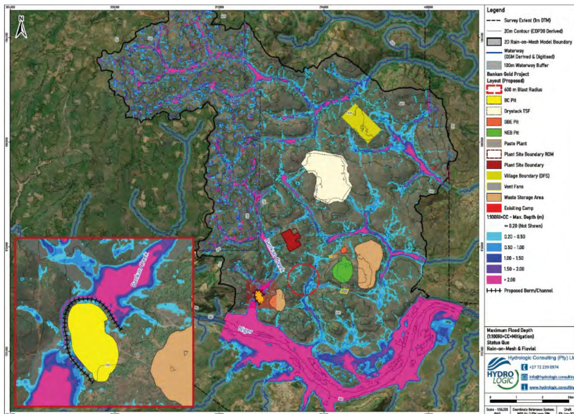
Figure 18.4: Flood Modelling Outcomes 1:100 RI plus Climate Change Event
