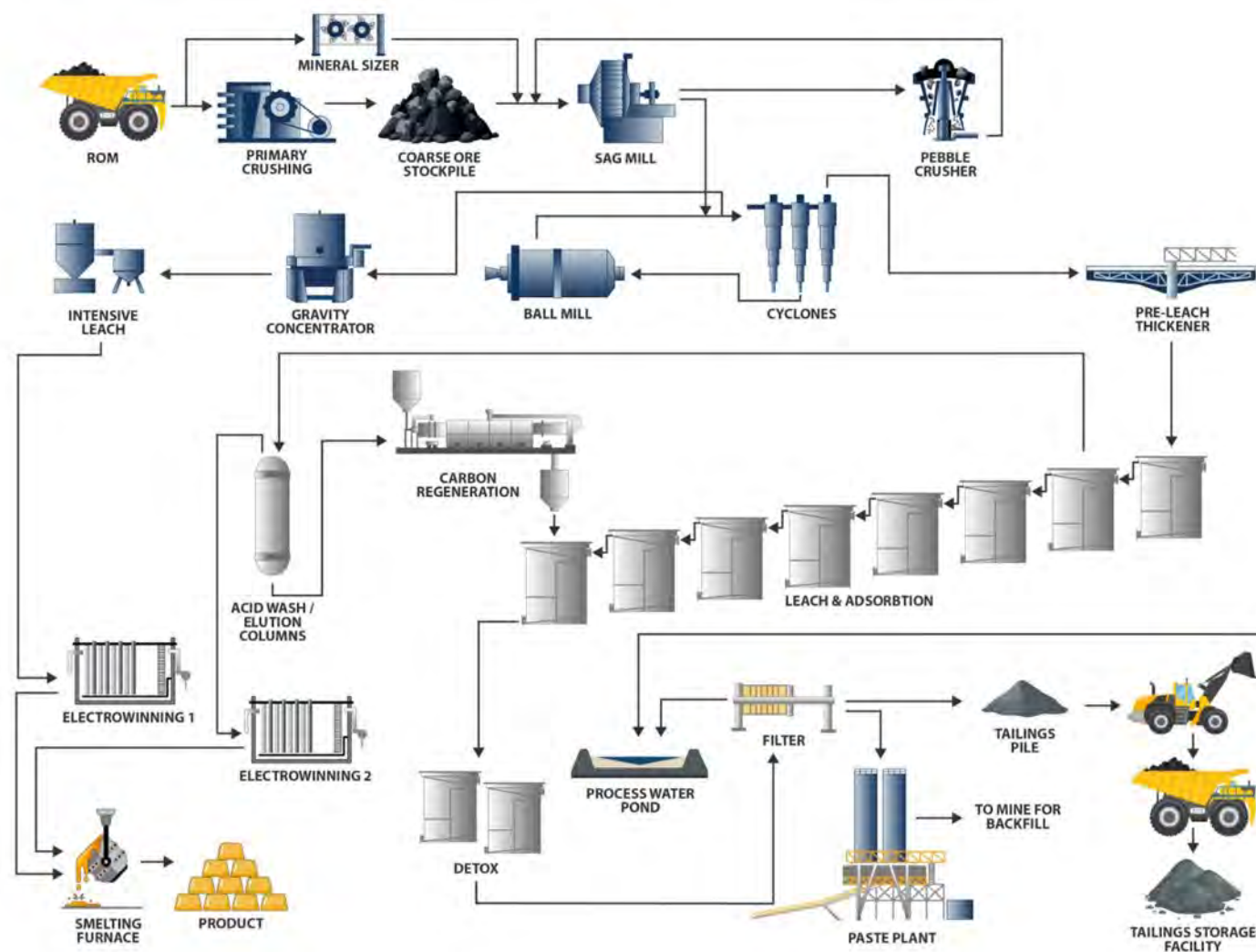
Figure 17.2: Process Flowsheet
