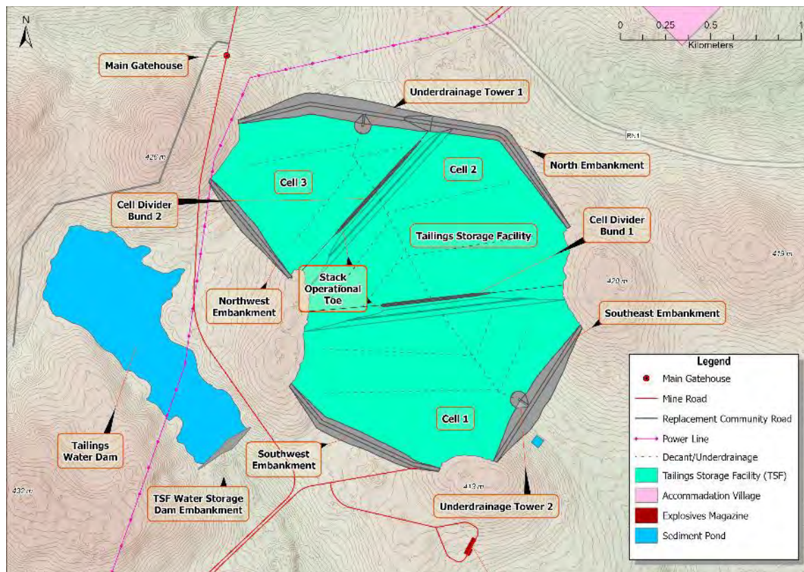
Figure 18.2: TSF and Tailing Water Storage Dam
