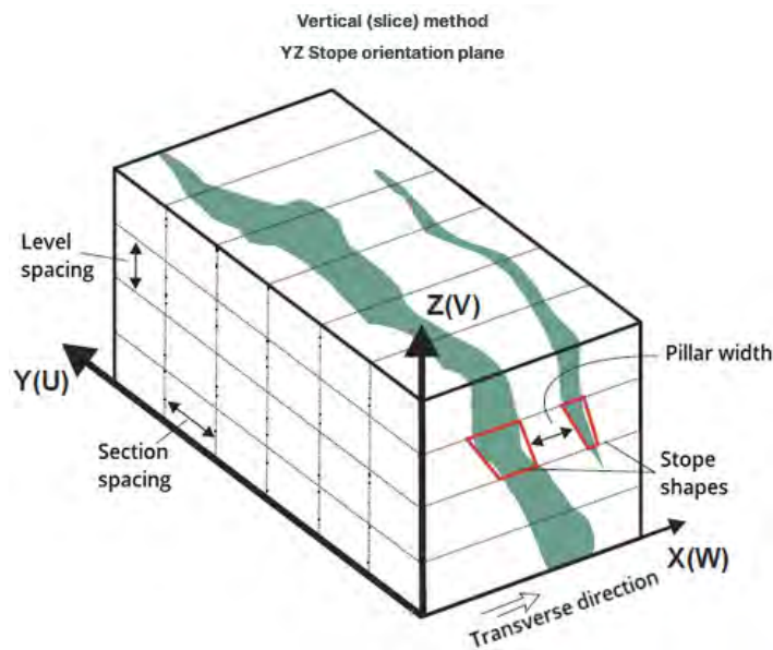
Figure 15.14: Vertical Slice Method Applied to a Vertical Orebody (Orelogy 2025)
